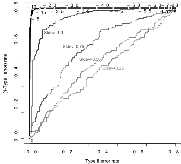
FIG. 2.—Evaluation of importance sampling estimates of the marginal likelihood to compare diffusion model fit. The thick black curve summarizes the two-by-two comparisons of BD and RRW models from which the over-dispersed diffusion was simulated using a lognormal distribution with a standard deviation of 1.7. The open circle symbols along the thick black curve represent different Bayes factor cutoff values. The four different precision matrix parameterizations generated comparisons that resulted in very similar curves, making them appear as single result. Additional simulations of 100 data sets were generated using lower lognormal standard deviations and one particular precision matrix ( p_1=7.7 , p_2 = 6.7 , r = 0.4 ).
