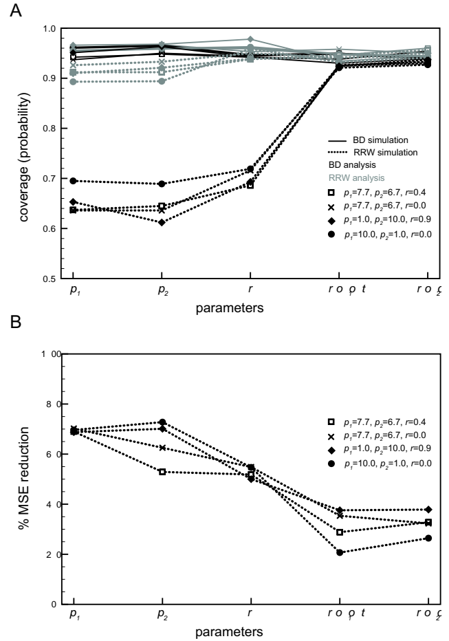
FIG. 1.—Results for a two-by-two simulation experiment that fits both the time-homogeneous Brownian diffusion (BD) and relaxed random walk (RRW) models to data simulated under homogeneous and over-dispersed diffusion. A. Estimator coverage for the precision matrix parameters and the root location realizations. B. Percentage reduction of the mean squared error (MSE) for the RRW over the BD models when fitting to over-dispersed data.
