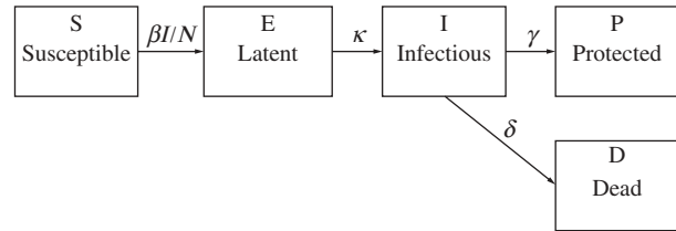
Fig. 2. Compartmental model indicating the transition of individuals among the different epidemiological stages during an influenza outbreak. \beta =transmission rate; N =total population; 1/\kappa =latent period; 1/\gamma =recovery period; \delta =mortality rate (see Table for parameter values).
